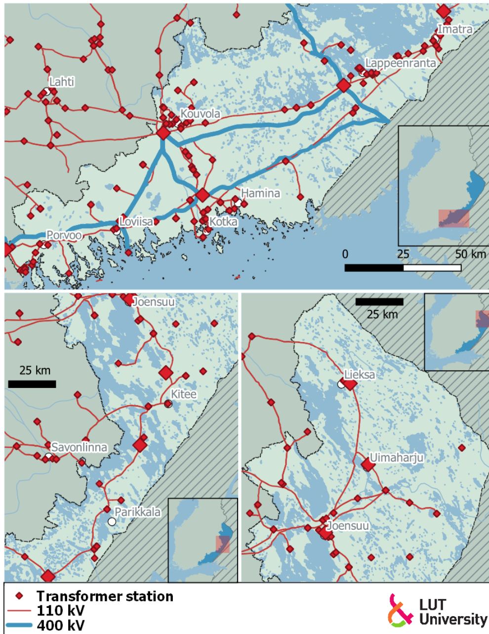
Figure 16. Existing electricity transmission grid and substations.
