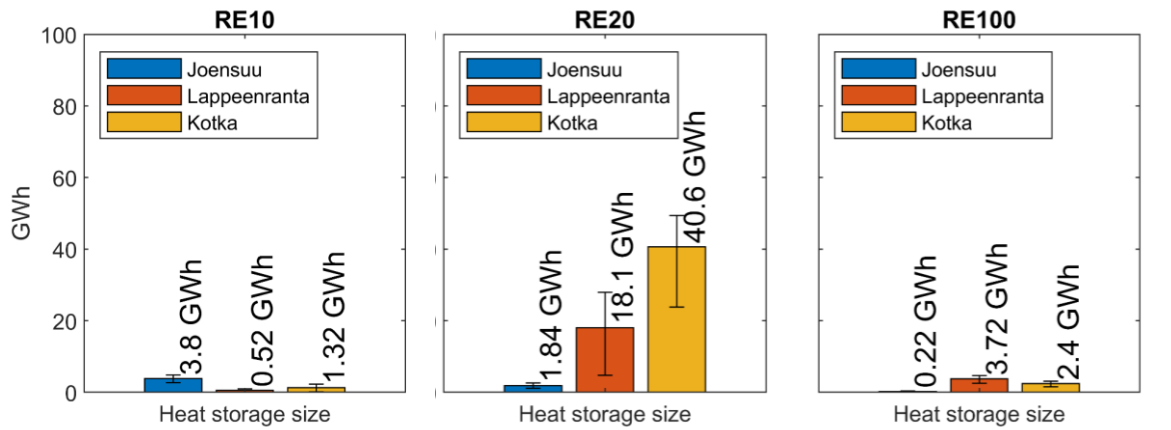
Figure 27. The average required heat storage capacity. Error bars represent the variation for different years 2016-2020.
